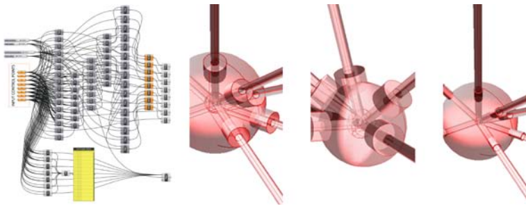
Figure 2: Grasshopper definition and parametric control of fabrication parameters
